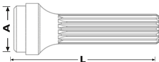
TYPE 1 FULL SPLINES
